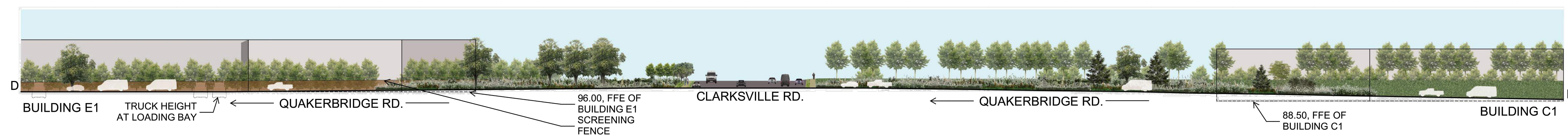
SECTION D-D' FROM QUAKERBRIDGE RD. - TREES AT MATURE SIZE
