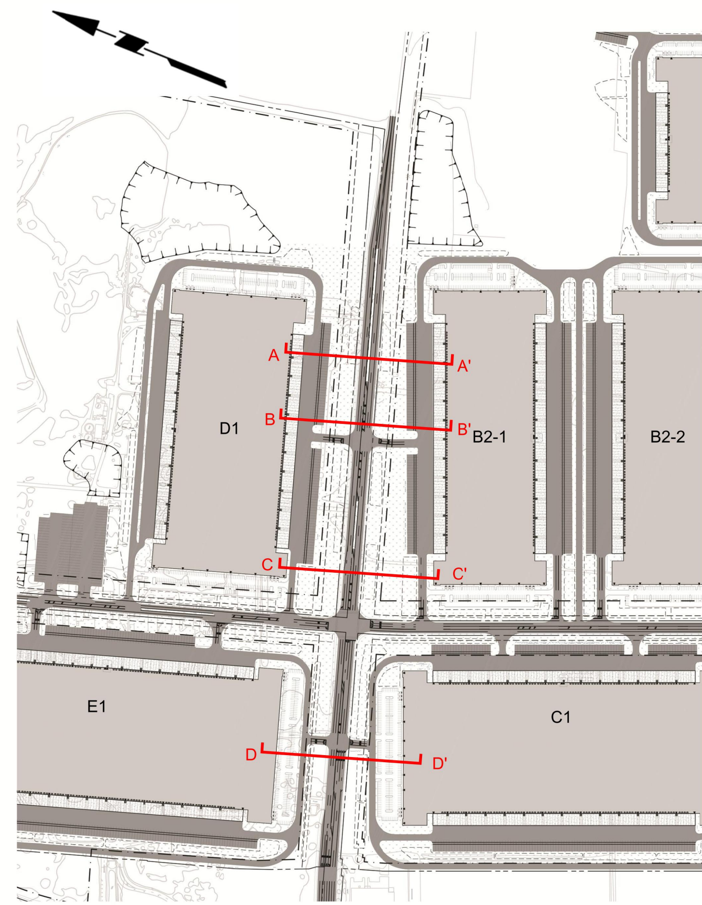
500 0 250 500 SCALE IN FEET Clarksville Road Section
